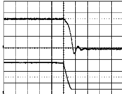
Shut-down enabled by disconnecting V_i at: T_{ref} = +25^{\circ}C , V_i = 53 V , I_o = 20 A resistive load. Top trace: output voltage (1 V/div.). Bottom trace: input voltage (20 V/div.). Time scale: (0.2 ms/div.).
