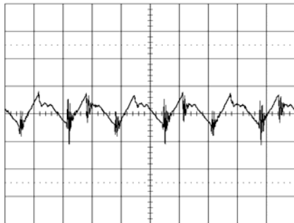
Output voltage ripple at: T_{ref} = +25^{\circ}C , V_i = 53 V , I_o = 20 A resistive load. Trace: output voltage (50mV/div.). Time scale: (2 \mu s/div.).
