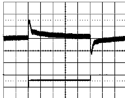
Output voltage response to load current step- Trace: output voltage (100mV/div.). change (5-10-5 A) at: T_{ref} = +25^{\circ}C , V_i = 53 V . Time scale: (0.1 ms/div.).
