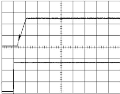
Start-up enabled by connecting V_i at: T_{ref} = +25^{\circ}C , V_i = 53 V , I_o = 20 A resistive load. Top trace: output voltage (1 V/div.). Bottom trace: input voltage (20 V/div.). Time scale: (10 ms/div.).
