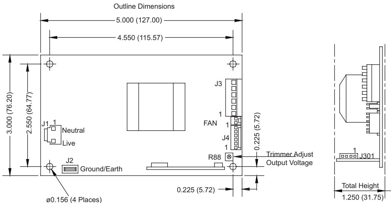
Figure 2: Mechanical Drawing
