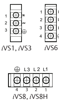
Figure 1. AC Input
