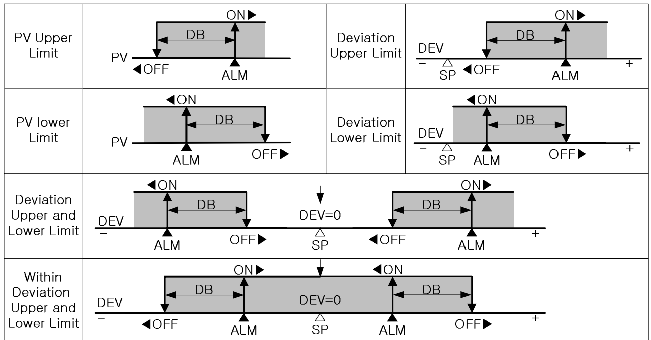
(Fig 8 : Alarm Operation)
