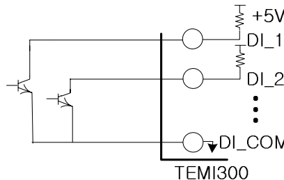
▲ TRANSISTOR contact input
