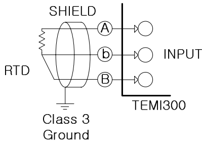
(A) RTD INPUT
