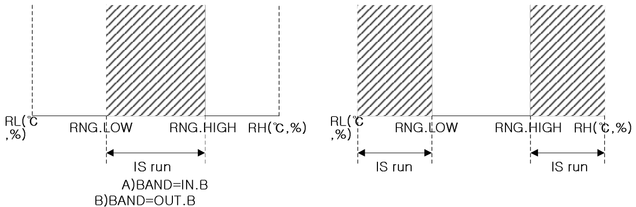
(Figure 7 : Ex. Inner Signal Zone)
