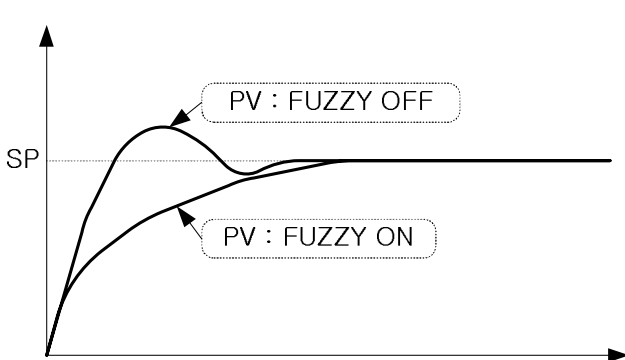
(Figure 1 : Overshoot suppressing function by FUZZY)
