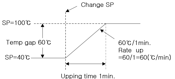
(Figure 2 : Ex. SLOPE setting)
