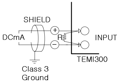
(C) DC CURRENT INPUT
