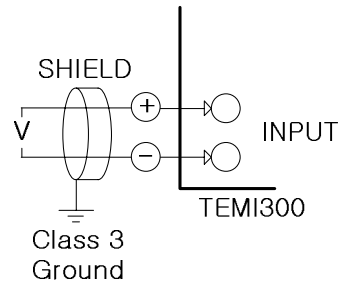
(B) DC VOLTAGE INPUT
