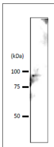
Fig.1. Detection of Srb4p in crude extract of S. cerevisiae by Western blotting
