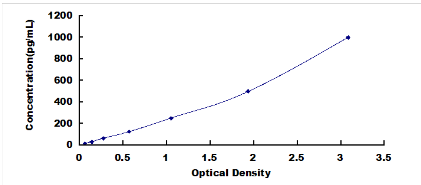
Typical Standard Curve for SEMG1, Human ELISA.
