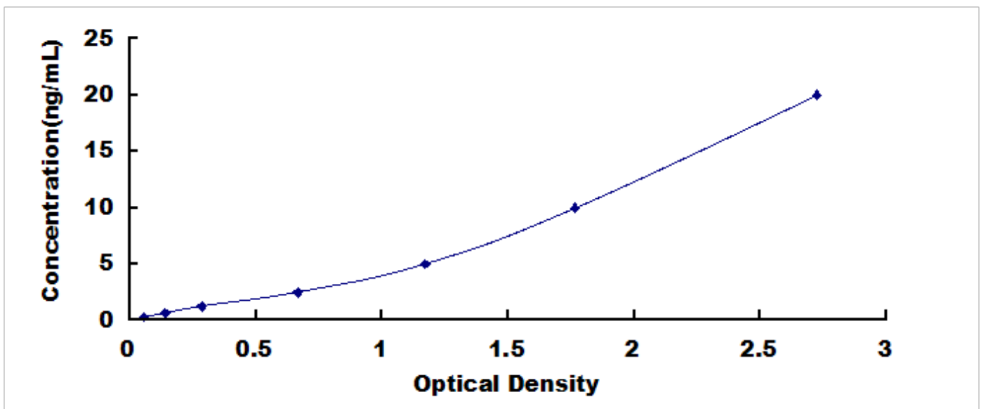
Typical Standard Curve for SEMA3E, Human ELISA.
