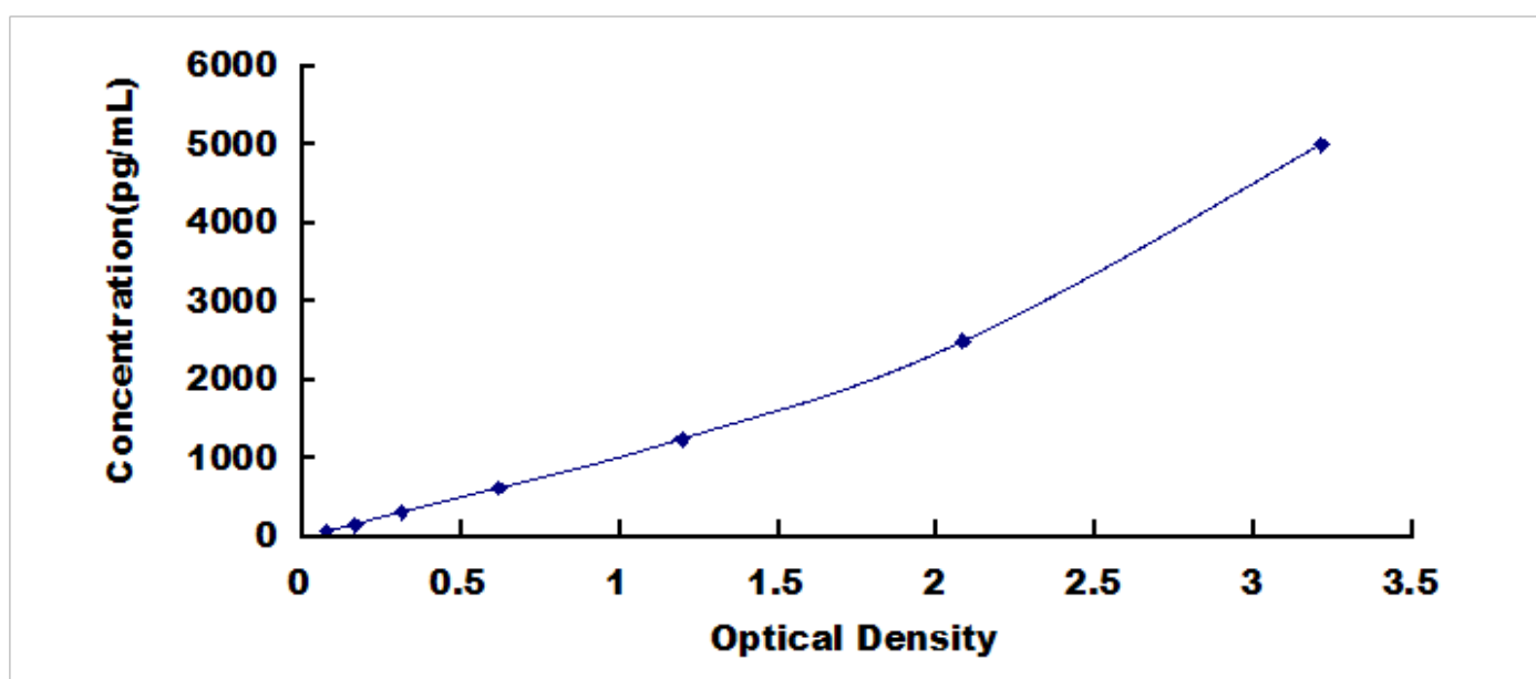
Typical Standard Curve for S100A6, Human ELISA.
