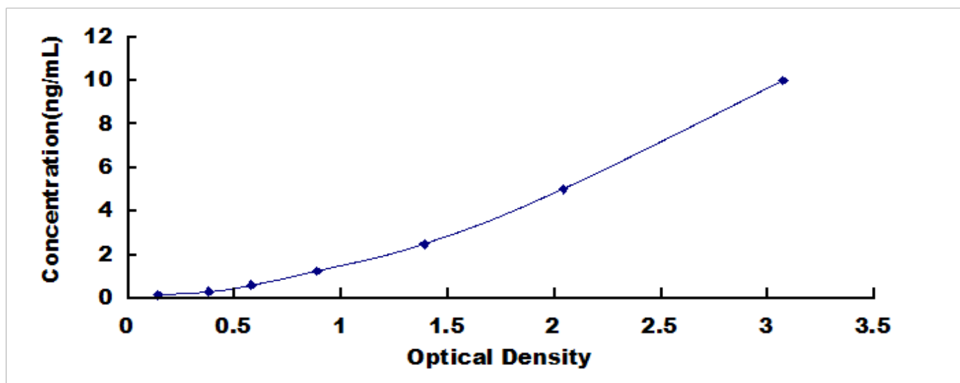
Typical Standard Curve for Noggin, Human ELISA.
