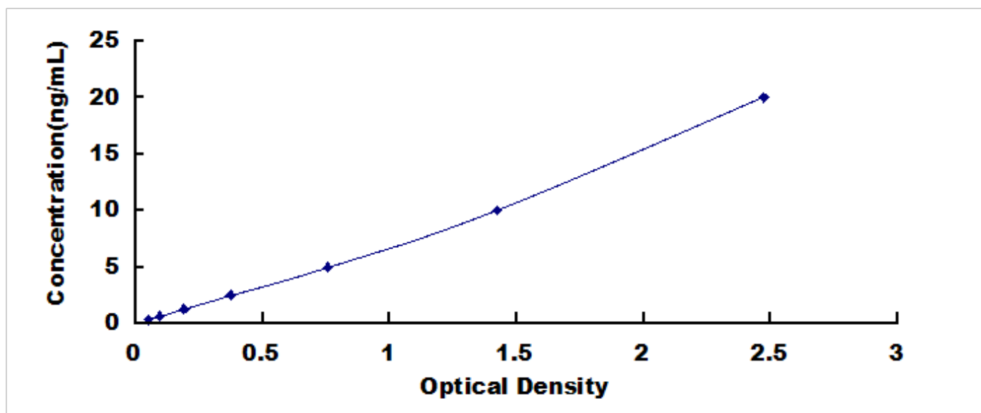
Typical Standard Curve for KIF5A, Human ELISA.
