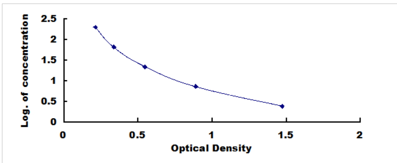
Typical Standard Curve for NTXI, Human ELISA.
