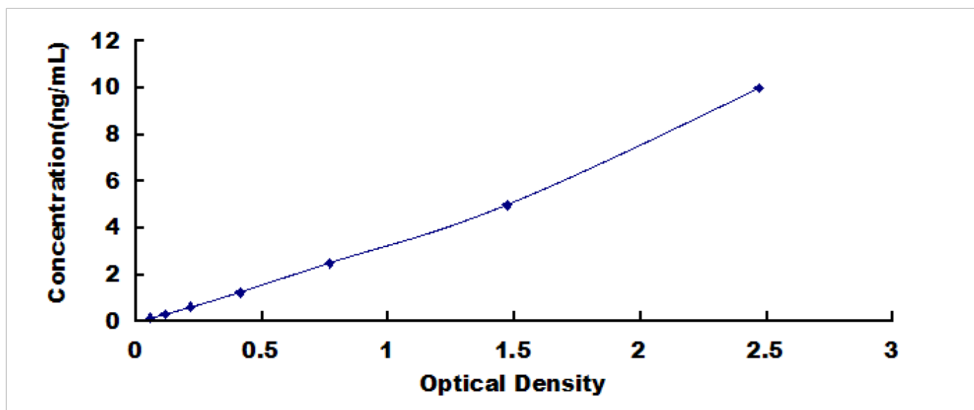
Typical Standard Curve for CTSG, Human ELISA.
