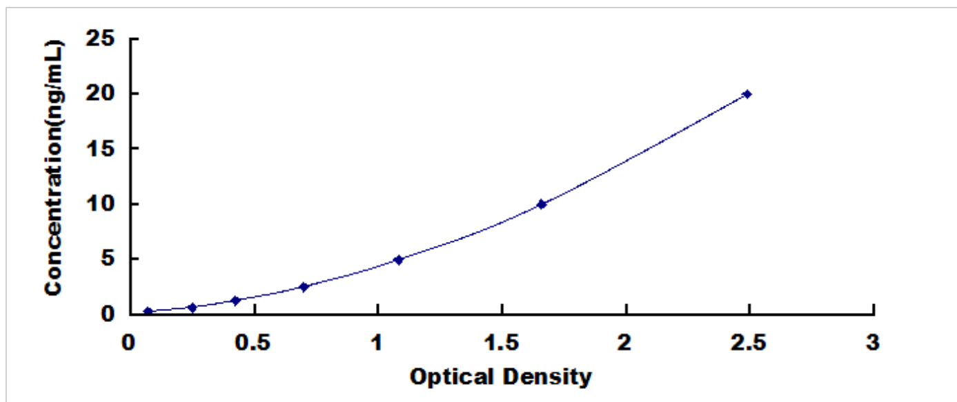
Typical Standard Curve for ATP2A2, Human ELISA.
