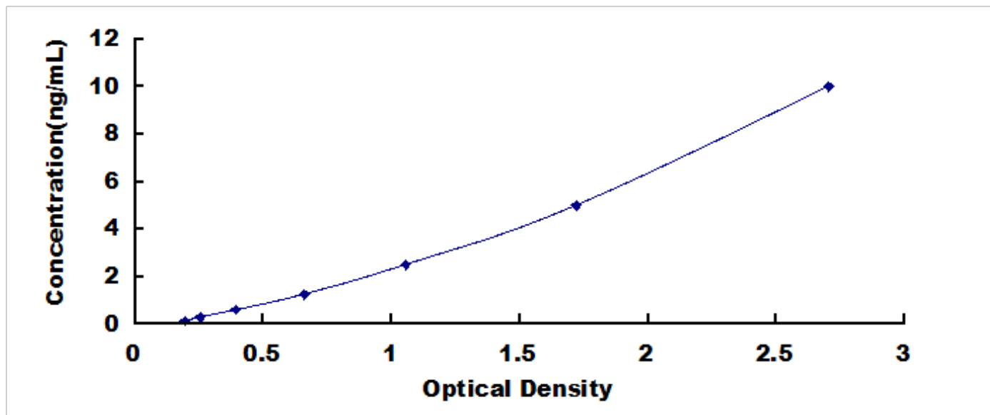
Typical Standard Curve for OAS3, Human ELISA.
