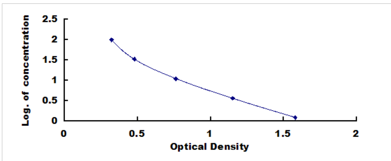
Typical Standard Curve for Glutathione ELISA.
