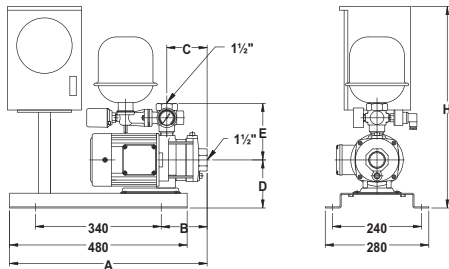
● 圖4. TPH4T4KICV ~ TPH4T6KICV
