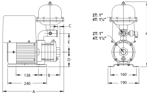
● 圖2. TPH2T - ICV
