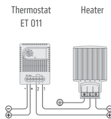
Heater
