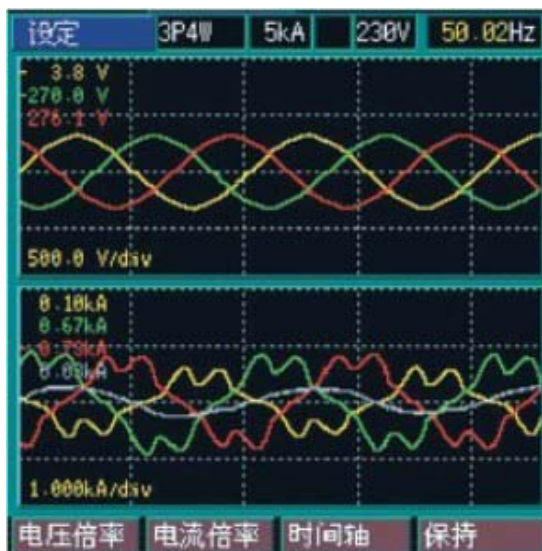
谐波治理前测试数据
