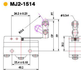
MJ2-1514 Micro switch, plastic body, IP67 MJ2-1514P Micro switch, phenolic body, IP67
