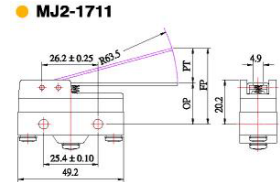
MJ2-1711 Micro switch, plastic body, IP67 MJ2-1711P Micro switch, phenolic body, IP67
