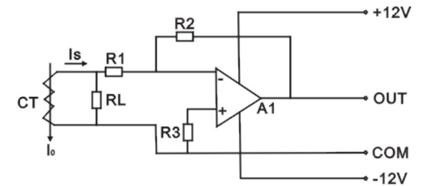
典型运用电路图 Typical application circuit
