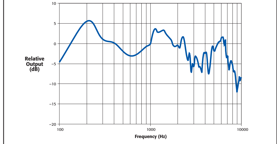
Figure 4. Frequency Response
