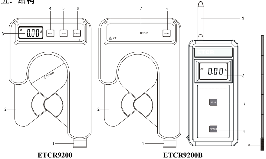
ETCR9200
