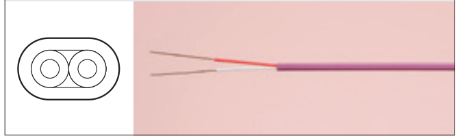
1 対平型FEP被覆 0.2×1P E-2-6F-J2 (0.2×1P E-6F)
