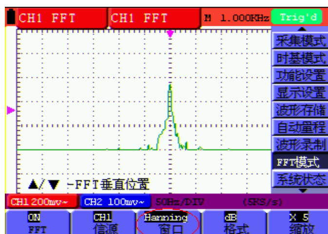
图62. HANNING 窗
