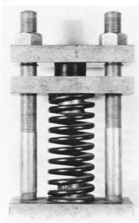
FIG. 2 Device for Compression Set Test, Using External Loading, Test Method A
