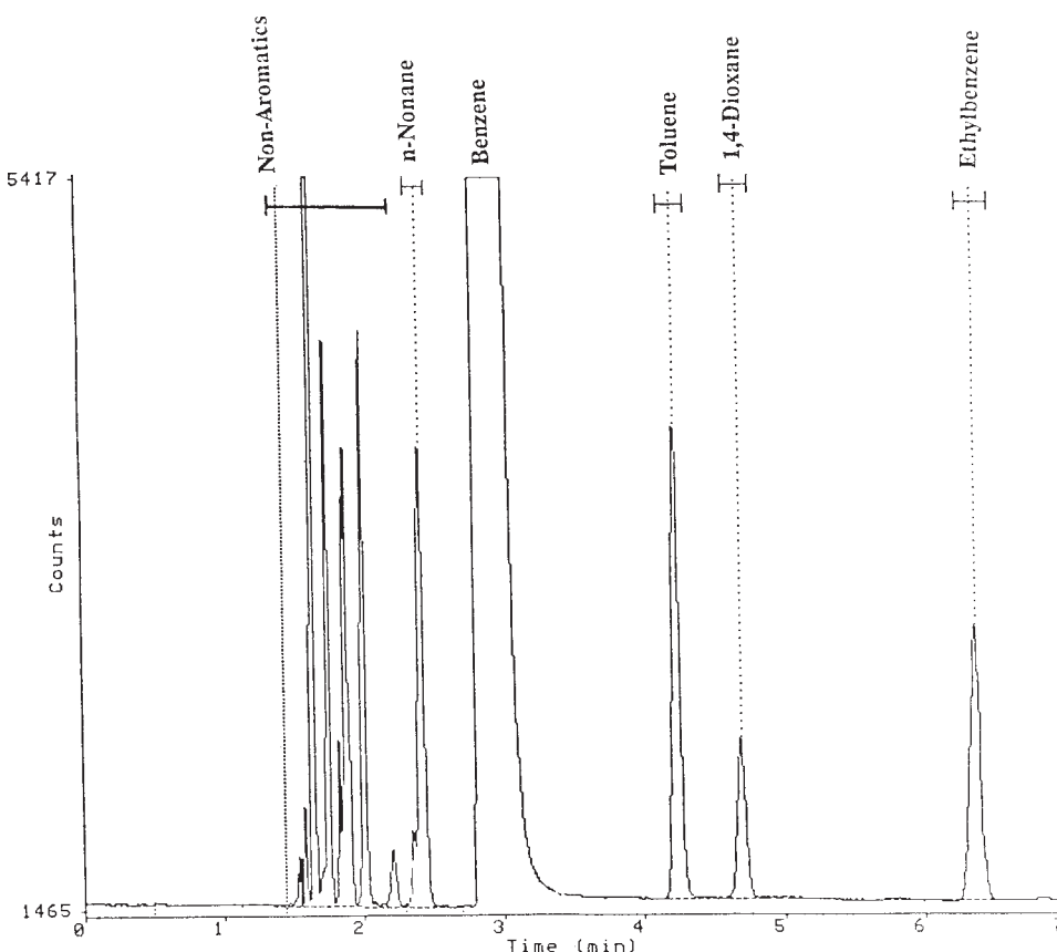
FIG. 1 Typical Chromatogram
