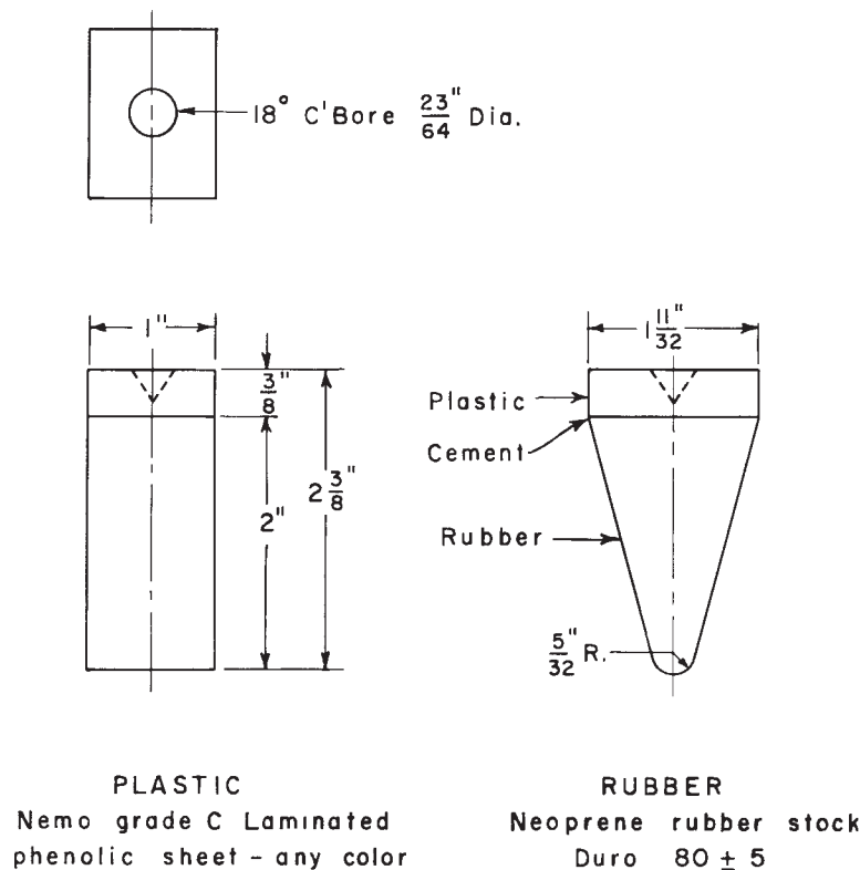
FIG. 2 Wedge Assemblies for Maeser Water Penetration Tester
