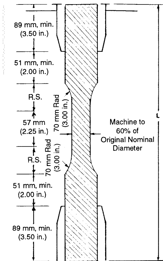
DIMENSIONS OF ROD SPECIMENS
