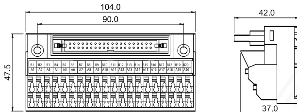
CONNECTOR(接线部)
