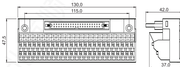
CONNECTOR(接线部)
