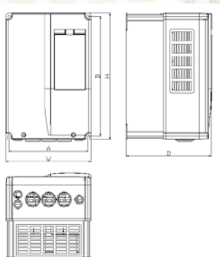
图 a EV3000-4T0022G ~ EV3000-4T0150G EV3000-4T0185G1 ~ EV3000-4T0220G1
