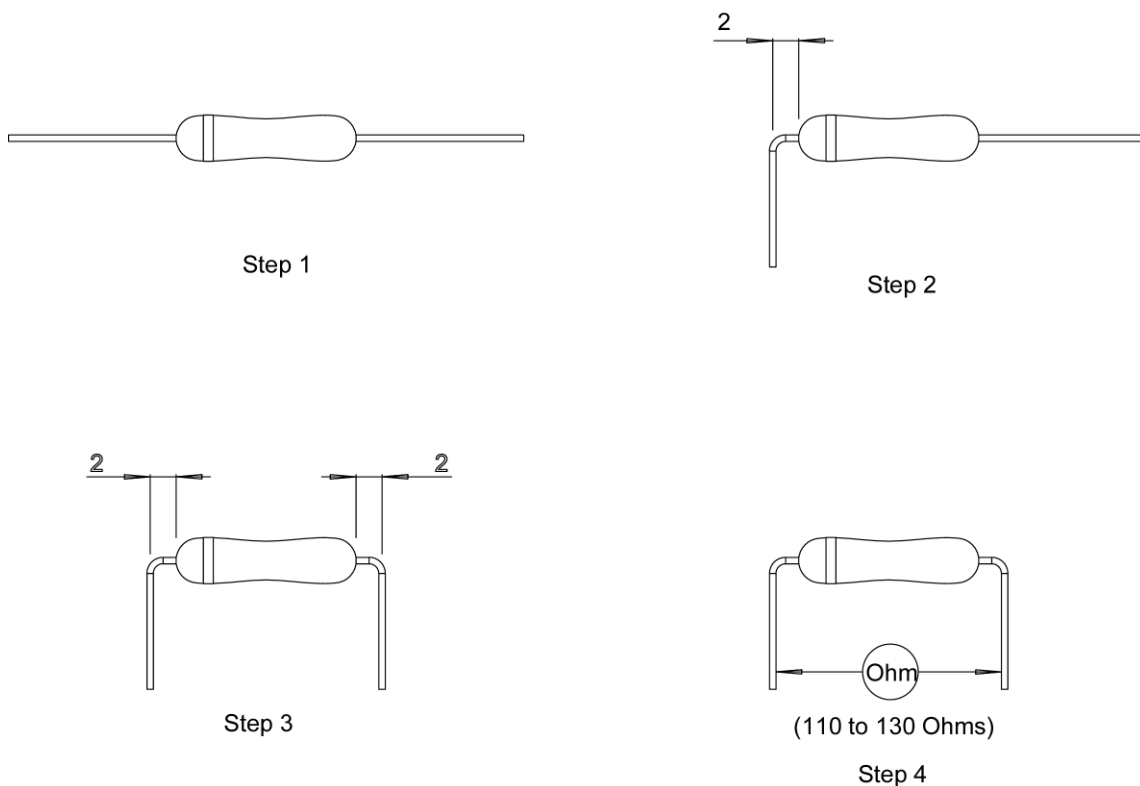
Figure 6. Sensor Lead Bending
