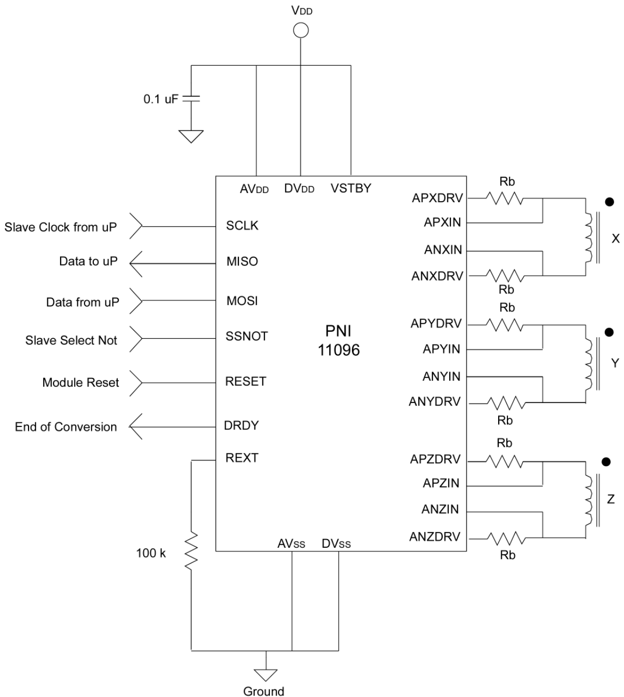
Figure 4. Block Diagram
