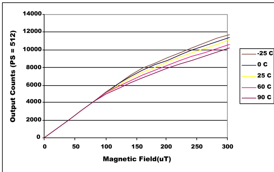
Figure 2. Linearity versus Temperature
