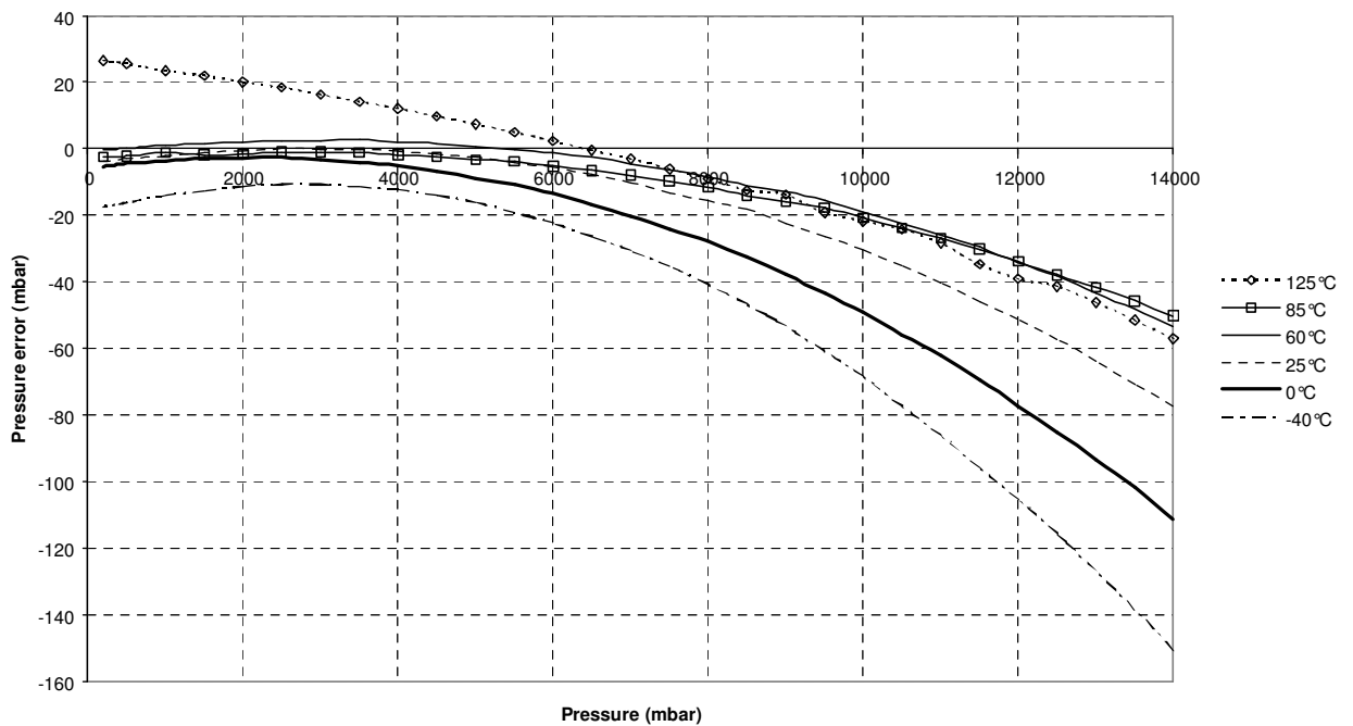
Absolute Pressure Accuracy (2nd order) after Calibration
